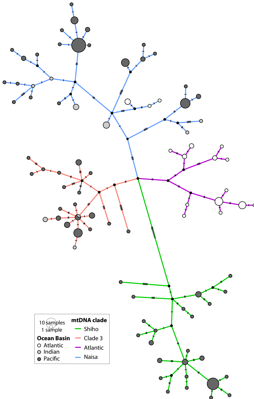
FIGURE 3 Median joining network (MJN) displaying the relationships among whole mitogenome haplotypes by ocean basin and mitogenomic clades. Circles are proportional in size to the number of samples with each haplotype. Cross hatches on lines indicate the number of differences between haplotypes. Missing haplotypes are indicated by a black node
